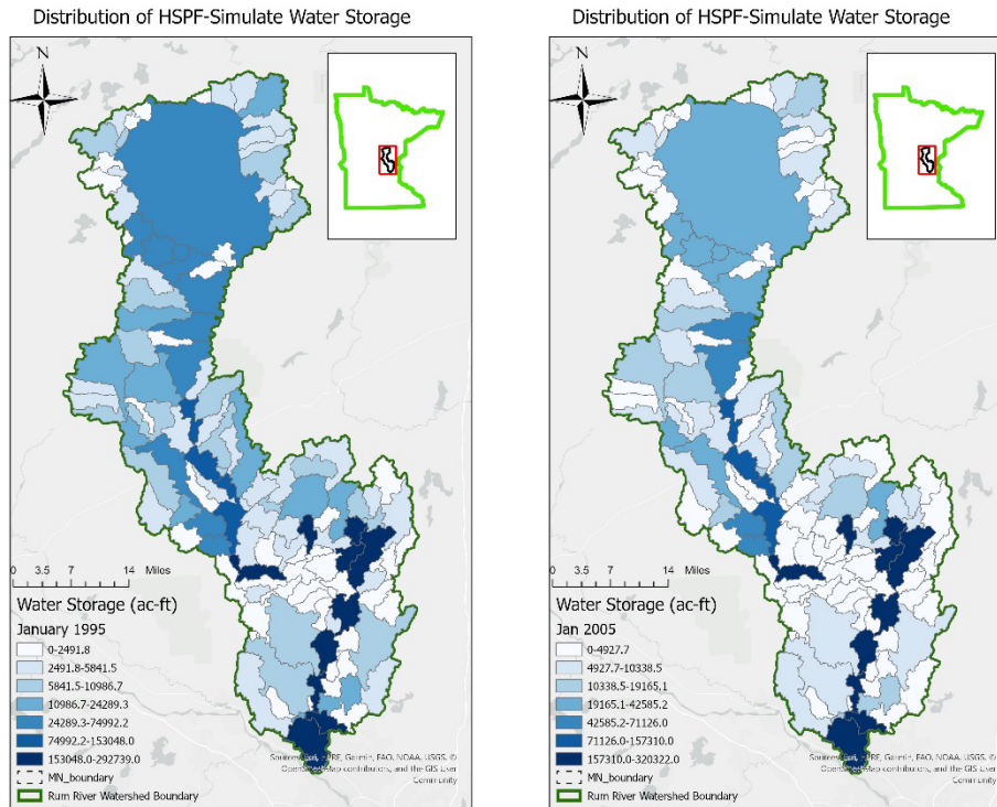
Figure 2. Distribution of water storage in the Rum River on two dates, Jan. 1995 and Jan. 2005.
