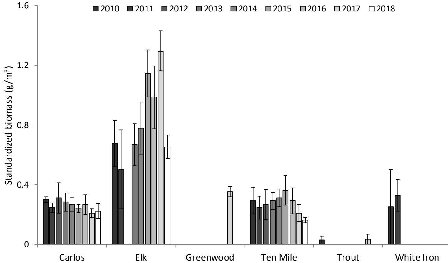
Figure 4. Standardized biomass ( \text{g}/\text{m}^3 ) for the lakes currently being sampled as part of the LTM program. Population estimates were standardized by the volume of water with a bottom depth > 6 m (Table 1).
